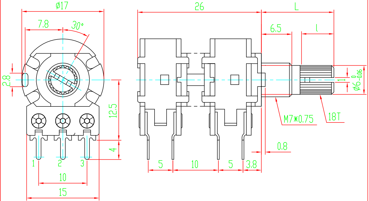
P.C.B MOUNTING DETAIL
