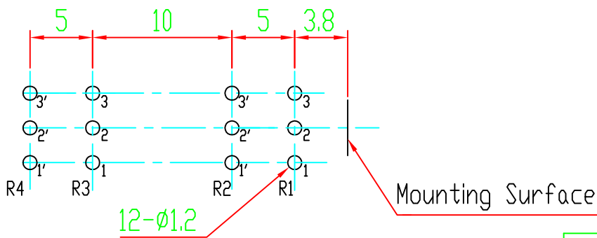
P.C.B MOUNTING DETAIL
